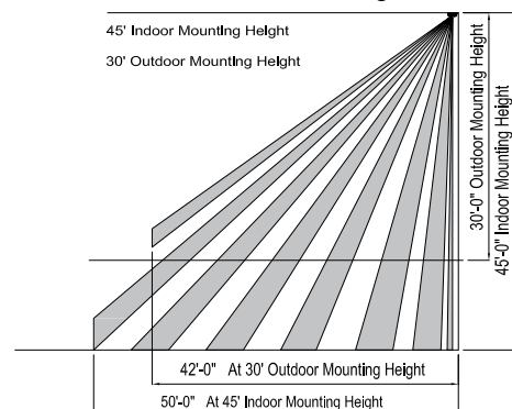
Fig. 7 – Side View of Lens Coverage Pattern at 30ft and 45 ft
