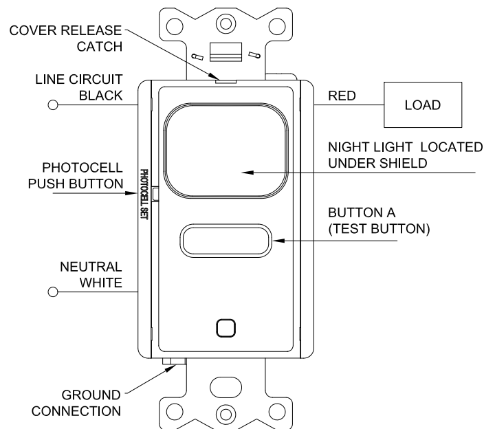
FIGURE I - WIRING DIAGRAM
